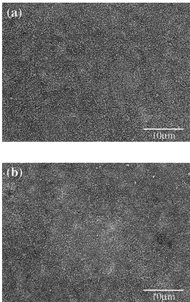
Fig. 3. SEM photographs of \beta - \text{Si}_3\text{N}_4 fabricated from submicrometer \beta -powder hot-pressed at 1800°C for 30 min: (a) planes parallel and (b) planes perpendicular to hot-pressing surface.
