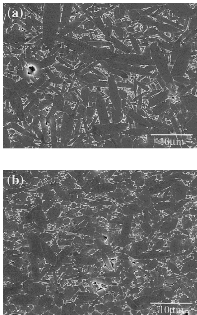
Fig. 4. SEM photographs of \beta - \text{Si}_3\text{N}_4 fabricated from SN-E10 hot-pressed at 1800°C for 2 h, then annealed at 1850°C for 4 h: (a) planes parallel and (b) planes perpendicular to hot-pressing surface.
