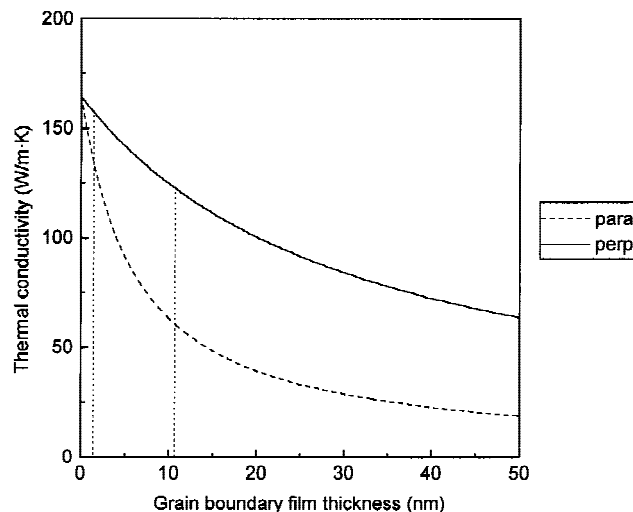
Fig. 8. Effect of grain-boundary thickness on thermal conductivity of \beta - \text{Si}_3\text{N}_4 for d = 1 \mu\text{m} , l = 5 \mu\text{m} ( R = 5 ), and x = 6\% .
