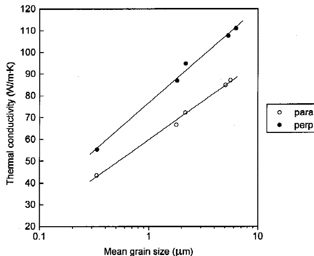
Fig. 6. Relationship between mean grain sizes and thermal conductivities of \beta - \text{Si}_3\text{N}_4 sintered bodies. Note: A straight line can be drawn for plots of experimental data when mean grain sizes are plotted using a logarithm scale.
