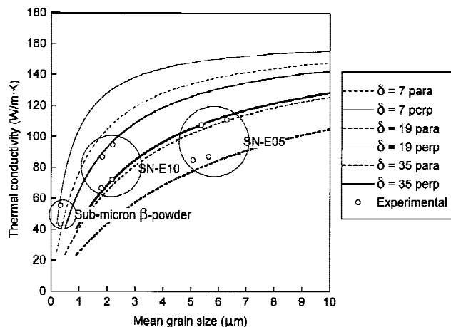
Fig. 11. Effect of grain size on thermal conductivity of \beta - \text{Si}_3\text{N}_4 with various grain-boundary film thickness values, comparing experimental data and best-fit calculations for R = 2 in \beta -grain and x = 6\% ; best-fit values of grain-boundary film thickness are 7, 19, and 35 nm for samples fabricated from submicrometer \beta -powder, SN-E10, and SN-E05, respectively.
