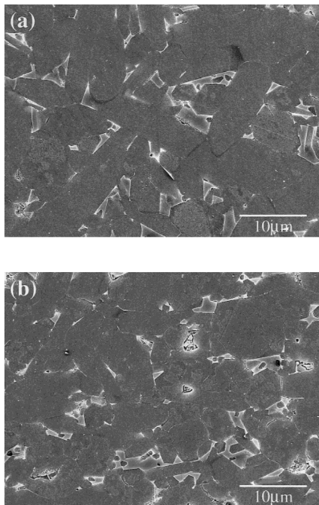
Fig. 5. SEM photographs of \beta - \text{Si}_3\text{N}_4 fabricated from SN-E05 hot-pressed at 1800°C for 2 h, then annealed at 1850°C for 4 h: (a) planes parallel and (b) planes perpendicular to hot-pressing surface.
