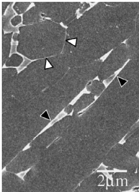
Fig. 7. Enlargement of SEM photograph in Fig. 3(a): Part of grain boundary indicated by ( \Delta ) is very thin, with equilibrium grain-boundary thickness; ( \blacktriangle ) is much wider because of faceting of prismatic planes of \beta - \text{Si}_3\text{N}_4 .
